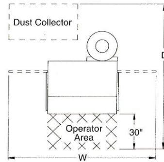
Floor Area Required Shown With 700 CFM Reclaimer
